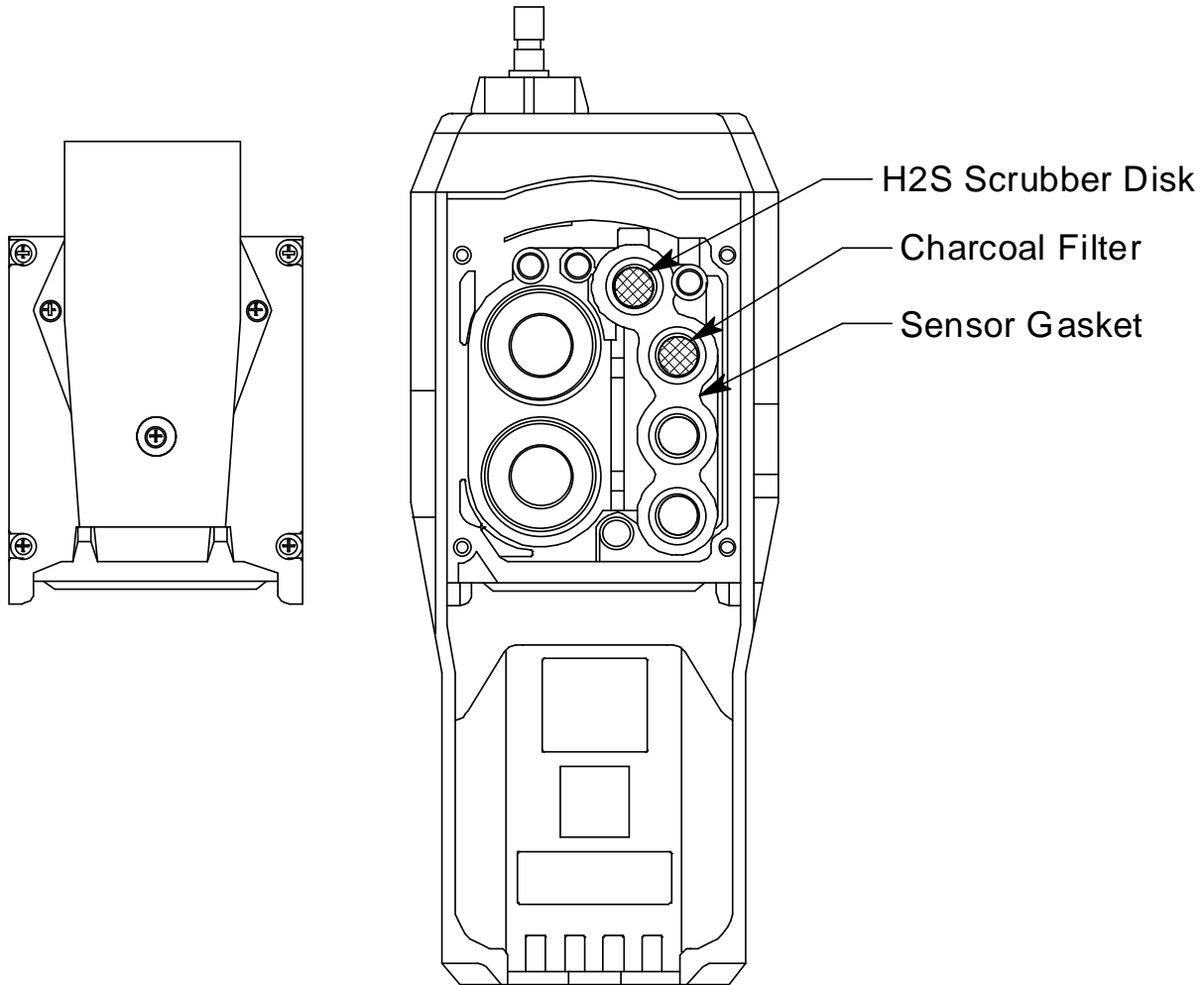
Figure 16: Replacing the H 2 S Scrubber Disk and Charcoal Filter
