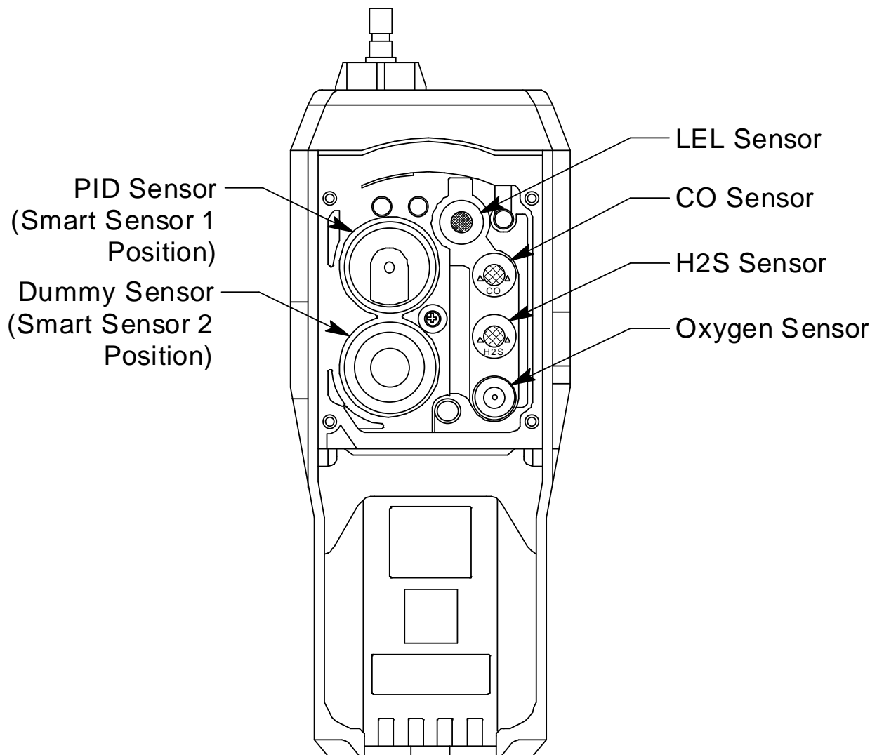
Figure 17: Replacing a Sensor
