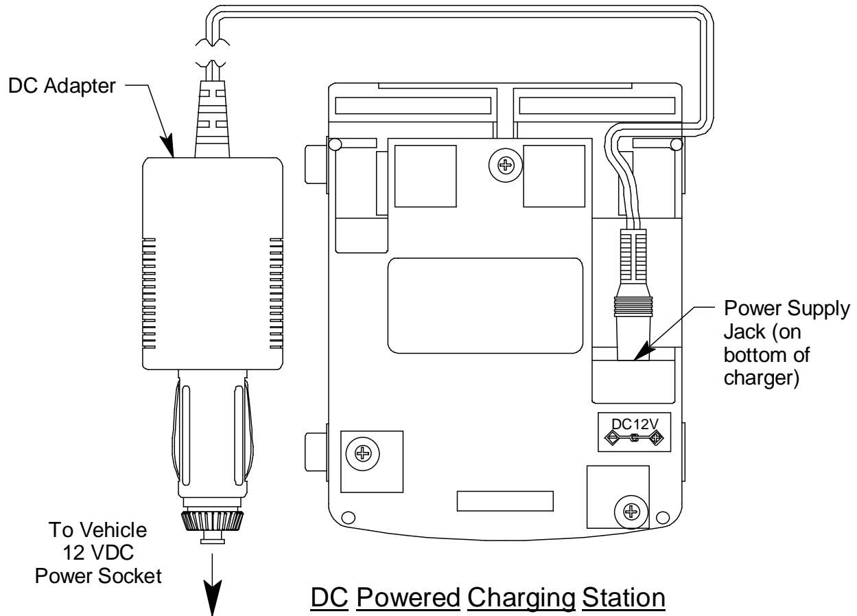
Figure 13: Connecting the Charging Station's DC Adapter
