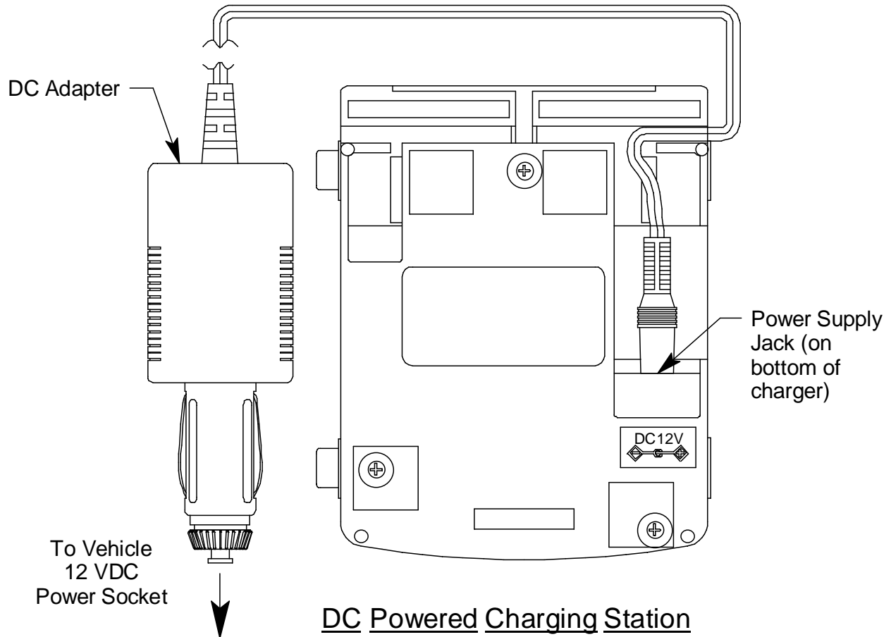
Figure 10: Connecting the Charging Station's DC Adapter
