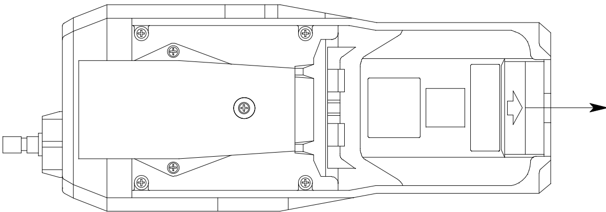
Figure 4: Releasing Battery Cover Latch
