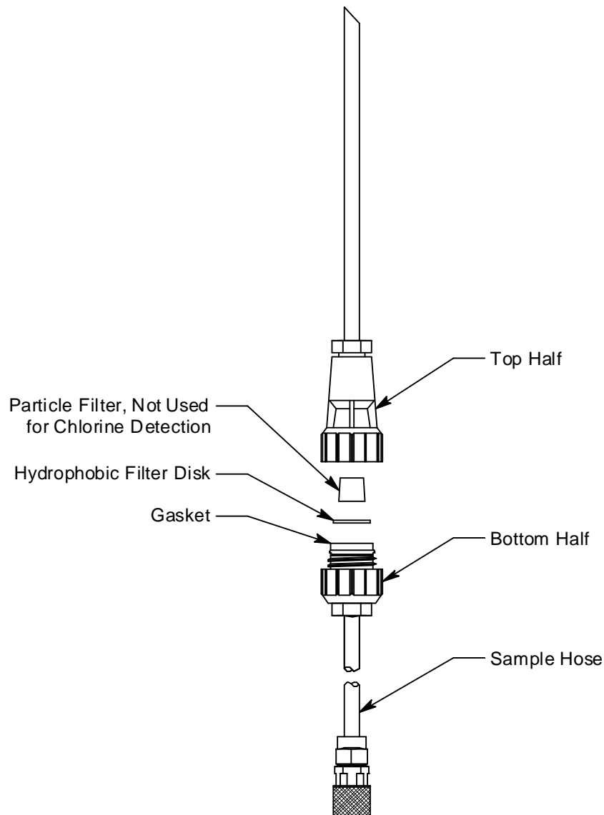
Figure 15: Replacing the Particle Filter and Hydrophobic Filter Disk
