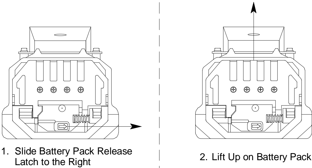
Figure 7: Releasing the Battery Pack
