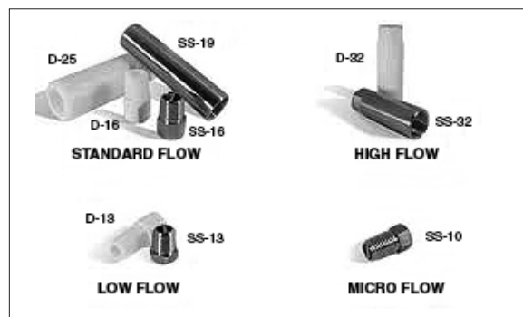
Foot Valves (w/part numbers)
