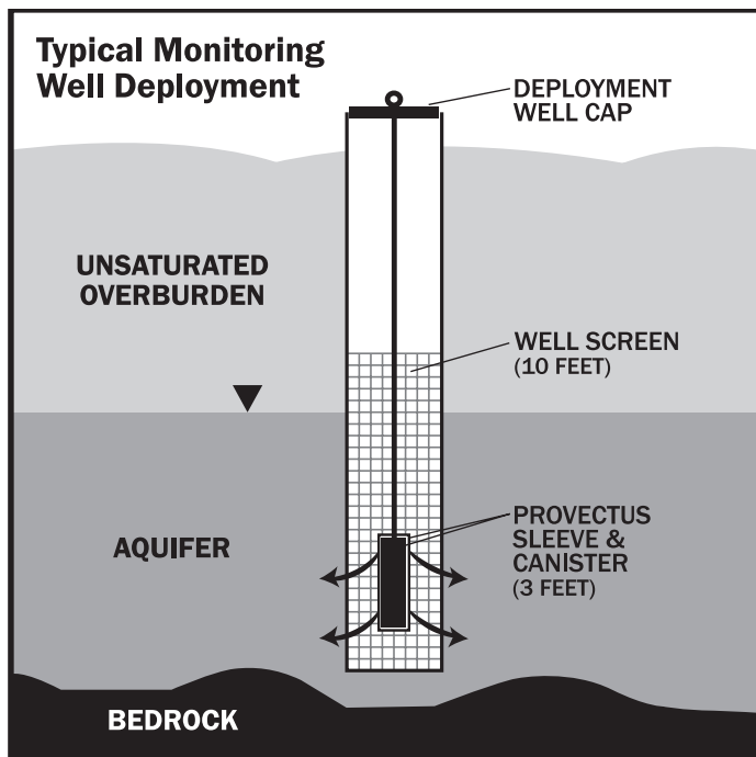
Provectus ORS™/ISCR Sleeve & Canister
