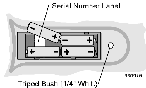
Figure 3: Battery orientation
