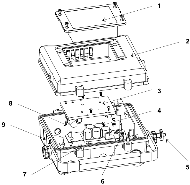
Figure 6-1 Main Components of SentryRAE
