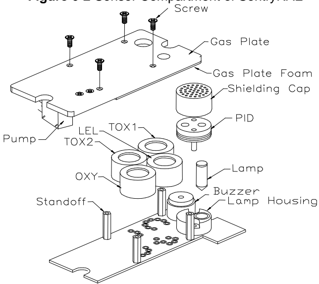
Figure 6-3 Detailed Sensor Assembly of SentryRAE
