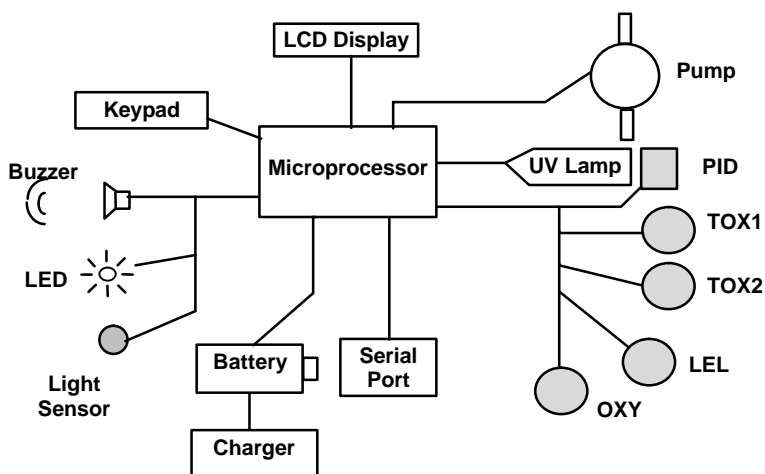
Figure 5-1 Block Diagram of SentryRAE Monitor
