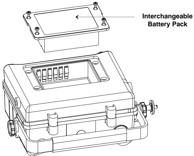
Figure 3-1. Interchangeable Battery Packs
