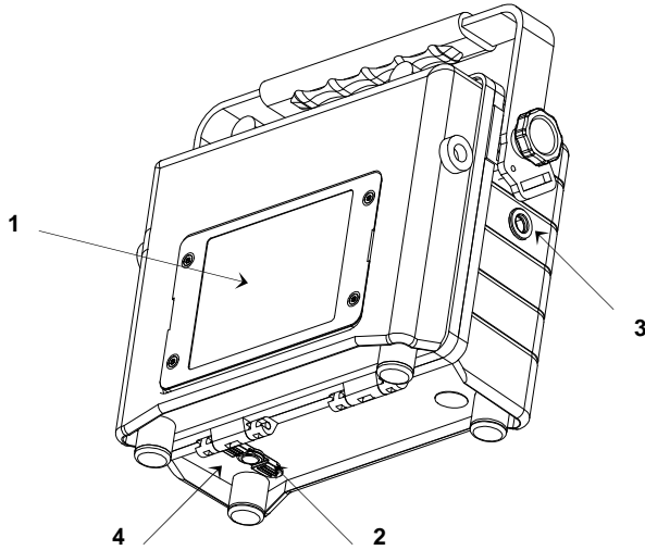
Figure 2-2 Back View - Main Components of SentryRAE
