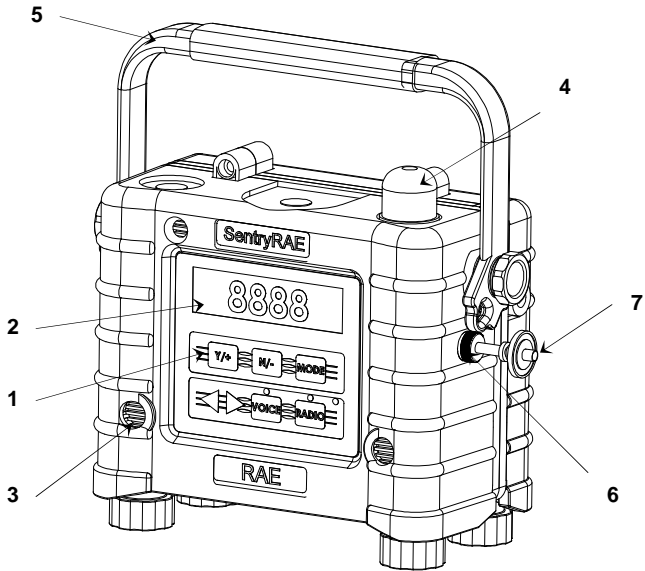
Figure 2-1 Front View - Main Components of SentryRAE
