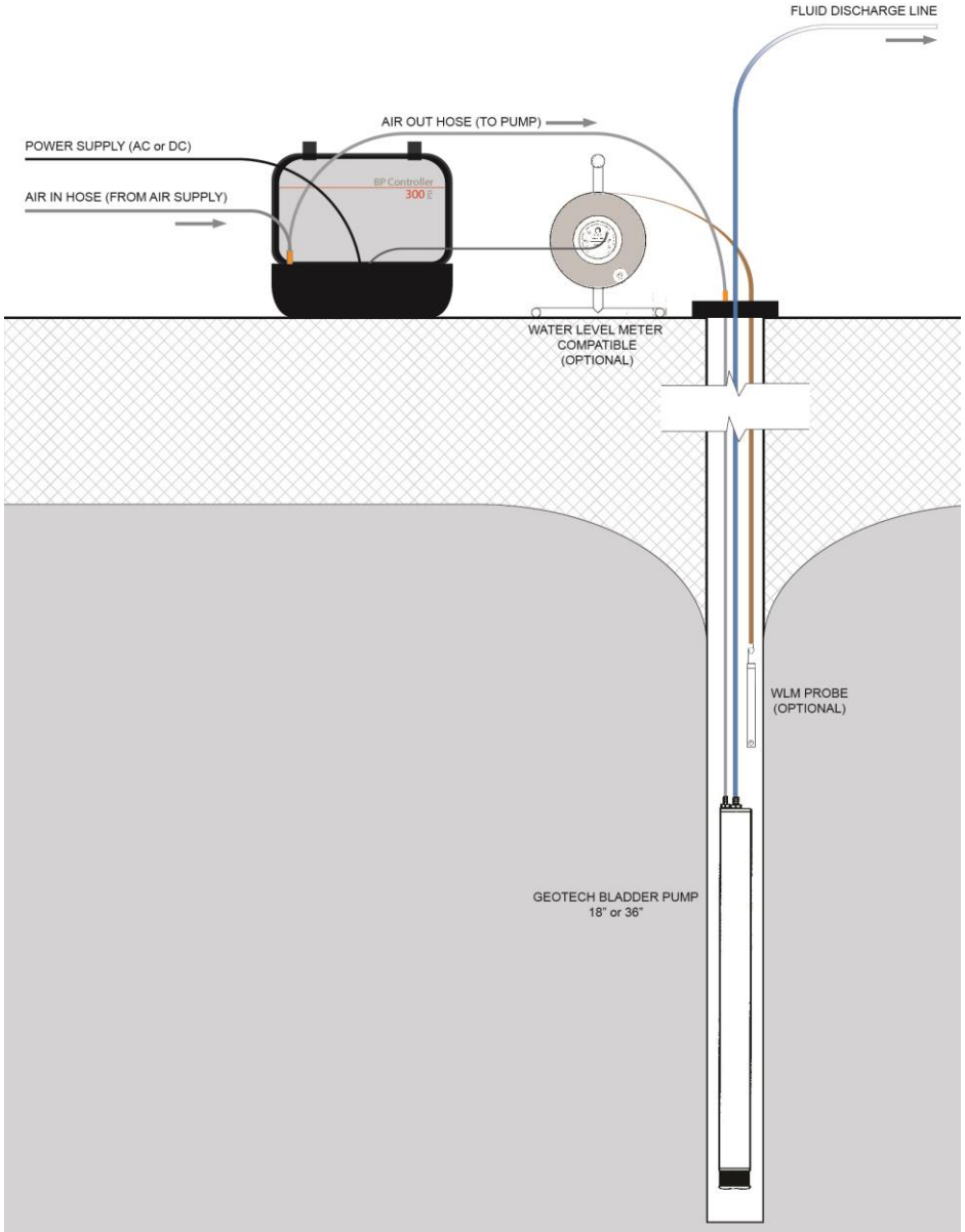
Figure 7.1 – Site Schematic
